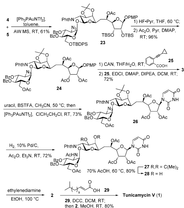
Scheme 3. Completion of the synthesis of tunicamycin V ( 1 ). AW MS = acid-washed molecular sieves, BSTFA = N , O -bis(trimethylsilyl)tri-fluoroacetamide, CAN = ceric ammonium nitrate, DCC = 1,3-dicyclohexylcarbodiimide, DIPEA = N,N -diisopropylethylamine, EDCI = 1-(3-dimethylaminopropyl)-3-ethylcarbodiimide hydrochloride.
