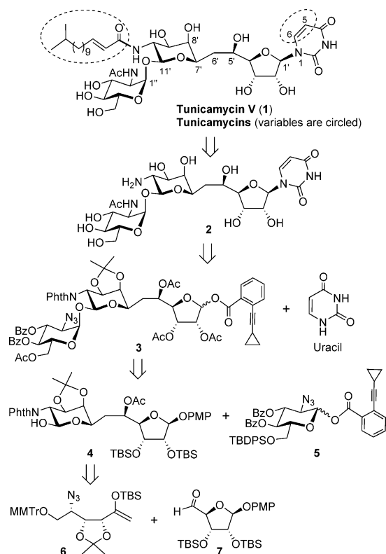
Figure 1. Tunicamycins and a retrosynthetic analysis. Ac = acetyl, Bz = benzoyl, Phth = phthaloyl, PMP = para -methoxyphenyl, TBDPS = tert -butyldiphenylsilyl, TBS = tert -butyldimethylsilyl.
