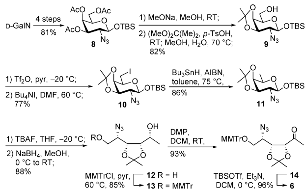
Scheme 1. Synthesis of silyl enol ether 6 . AIBN = 2,2'-azobis(isobutyronitrile), DCM = dichloromethane, DMP = Dess–Martin periodinane, MMTr = monomethoxytrityl, p -TsOH = para -toluenesulfonic acid, pyr = pyridine, TBAF = tetrabutylammonium fluoride, Tf = trifluoromethanesulfonyl.
