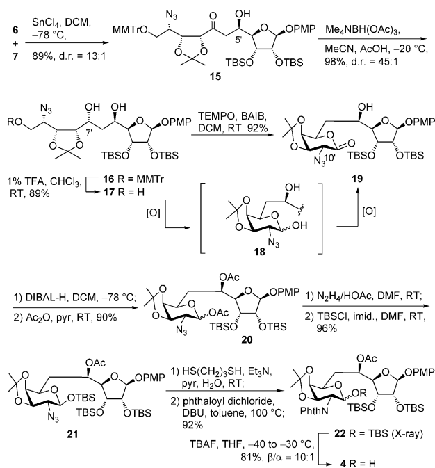
Scheme 2. Synthesis of undecose derivative 4 . BAIB = bis-(acetoxyl)iodobenzene, DIBAL-H = diisobutylaluminum hydride, TEMPO = 2,2,6,6-tetramethyl-1-piperidinyloxy, TFA = trifluoroacetic acid.
